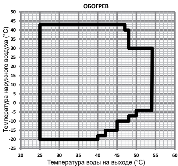
MDVM-V90D2BR8-A, MDVM-V180D2BR8-A
