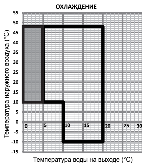
MDVM-V90D2BR8-A, MDVM-V180D2BR8-A
