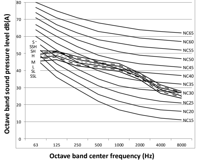
Figure 9.7: MDI2-200(250,280)T1DHN1 octave band levels
