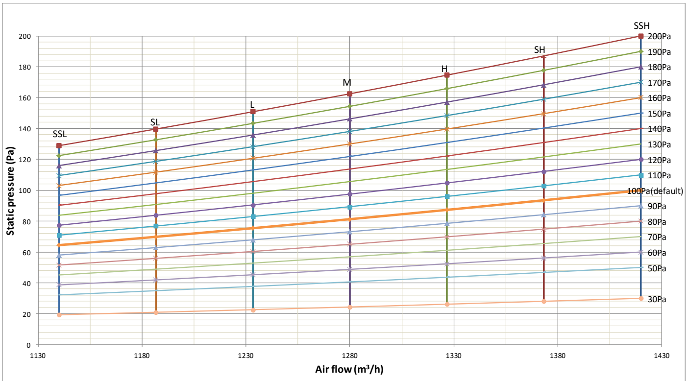
Figure 6.2: MDI2-90T1DHN1 fan performance
