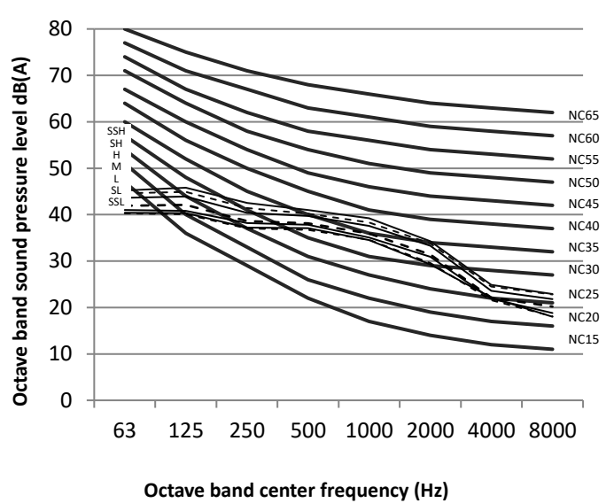
Figure 9.5: MDI2-140T1DHN1 octave band levels
