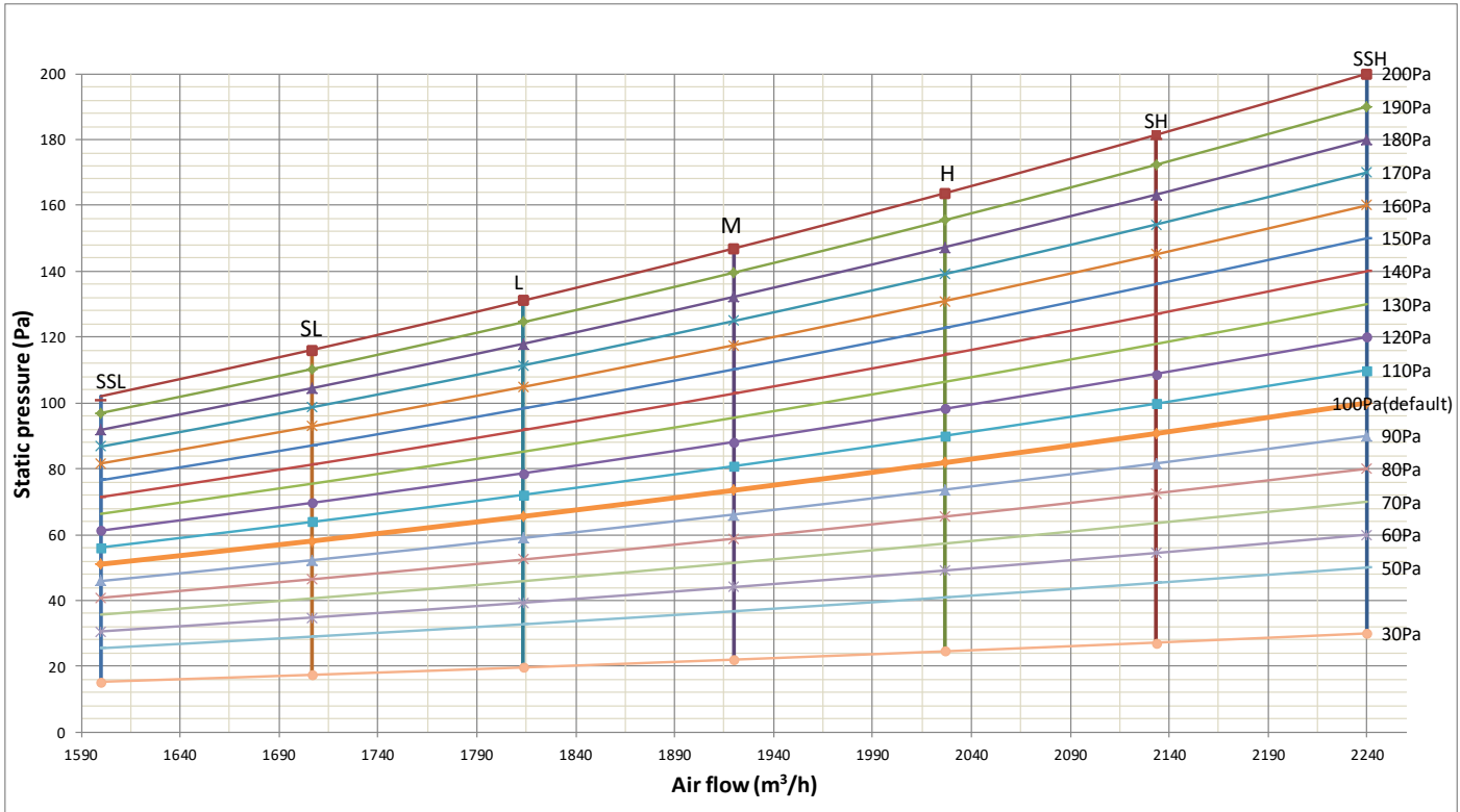
Figure 6.4: MDI2-140T1DHN1 fan performance
