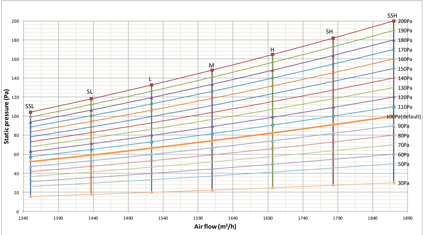
Figure 6.3: MDI2-112T1DHN1 fan performance
