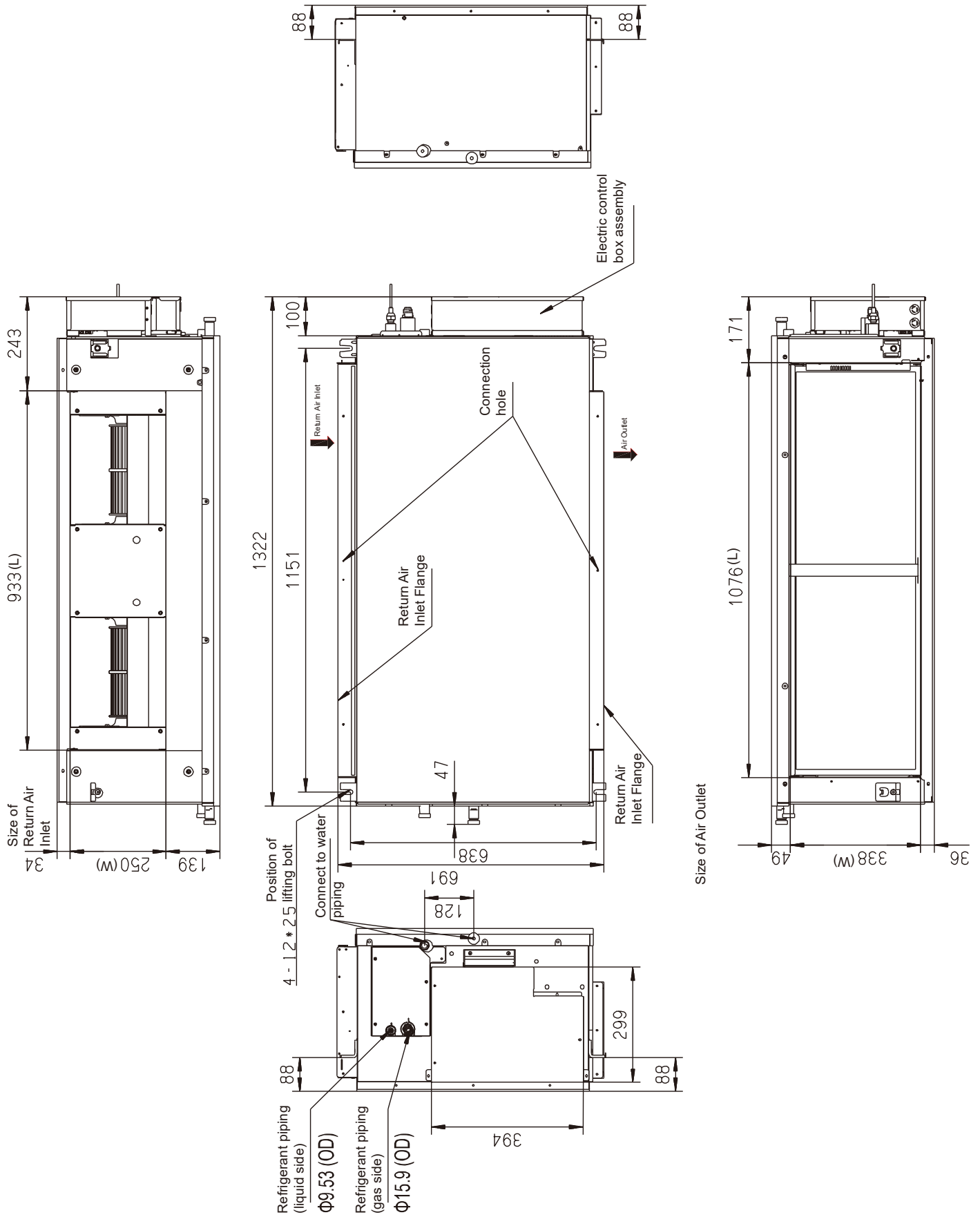
Figure 2.2: MDI2-140(160)T1DHN1 dimensions (unit: mm)
