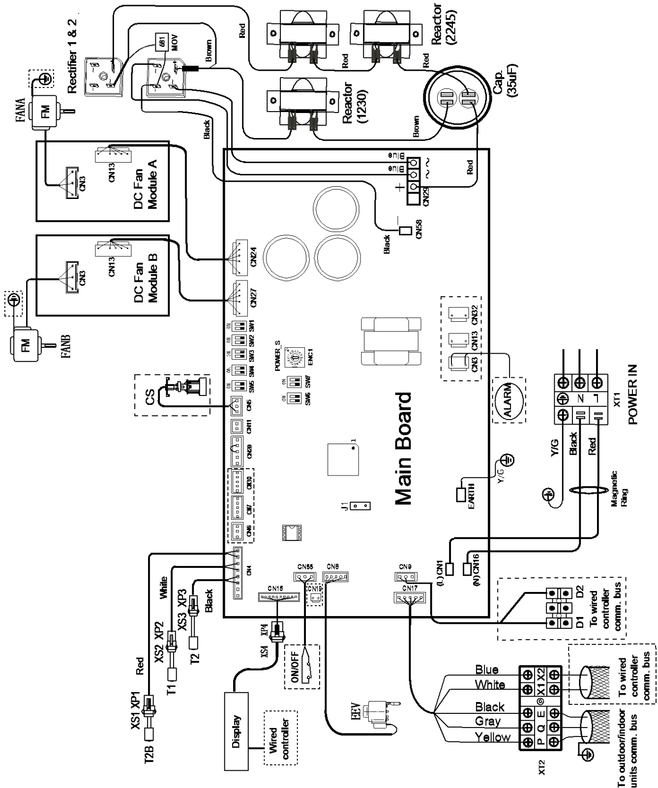
Figure 5.4: MDI2-400(450,560)T1DHN1 wiring diagram
