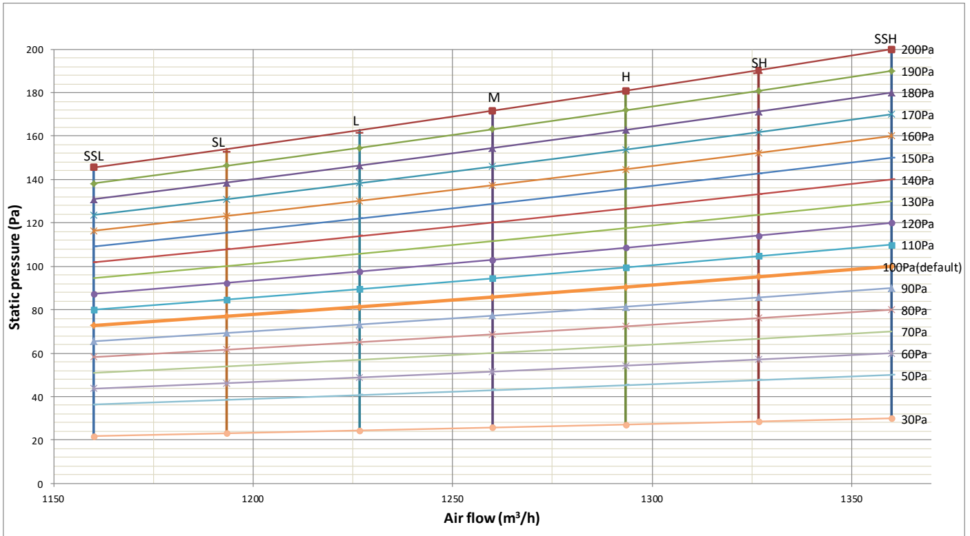
Figure 6.1: MDI2-71(80)T1DHN1 fan performance
