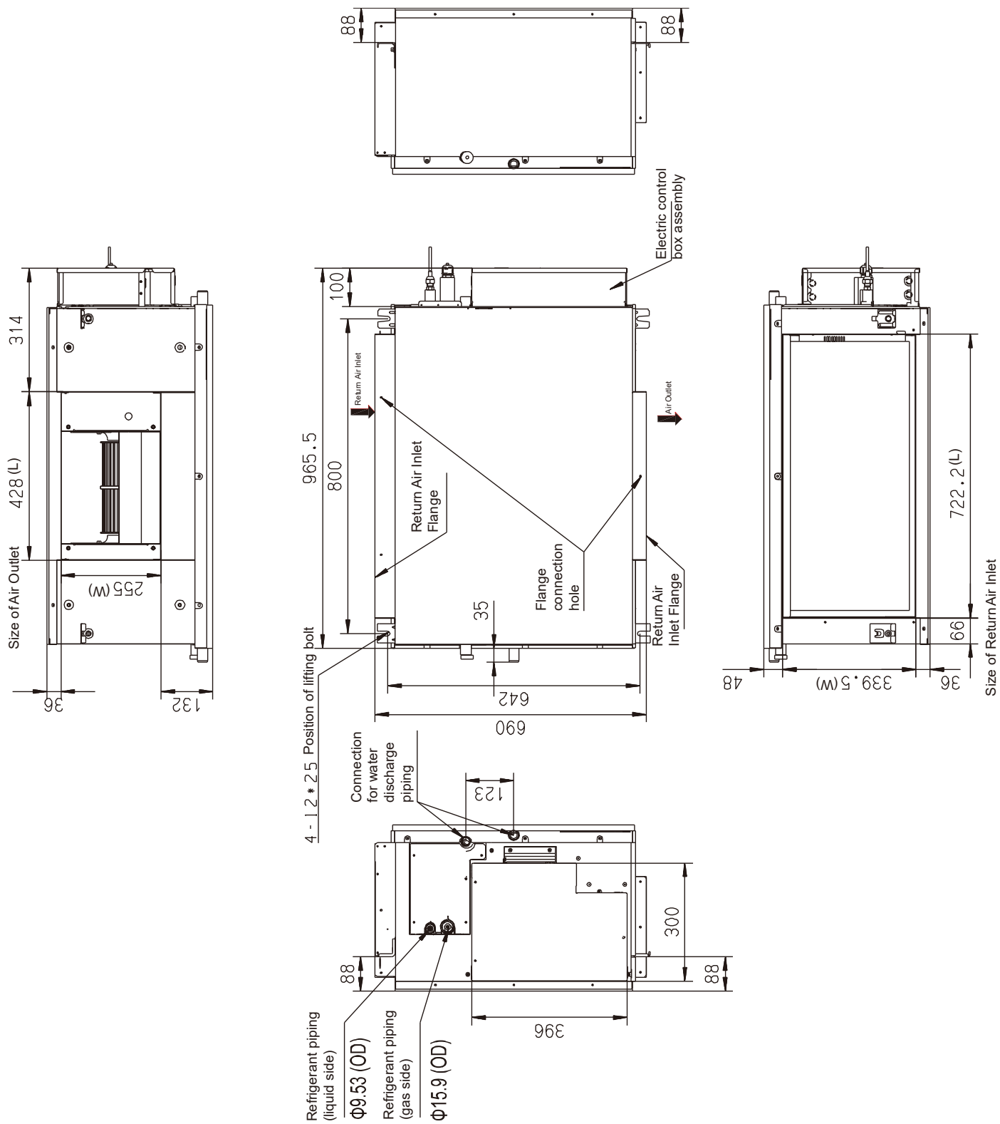
Figure 2.1: MDI2-71(80,90,112)T1DHN1 dimensions (unit: mm)
