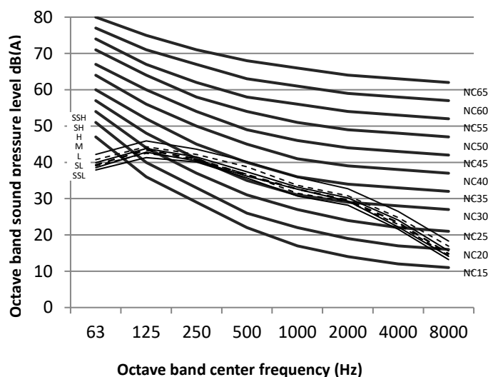
Figure 9.2: MDI2-71(80)T1DHN1 octave band levels
