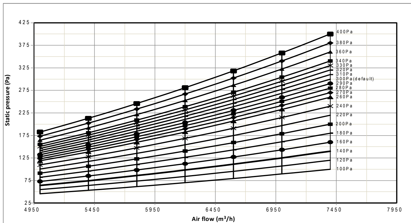
Figure 6.8: MDI2-560T1DHN1 fan performance
