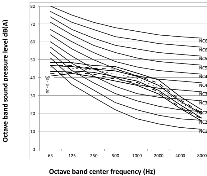
Figure 9.4: MDI2-112T1DHN1 octave band levels
