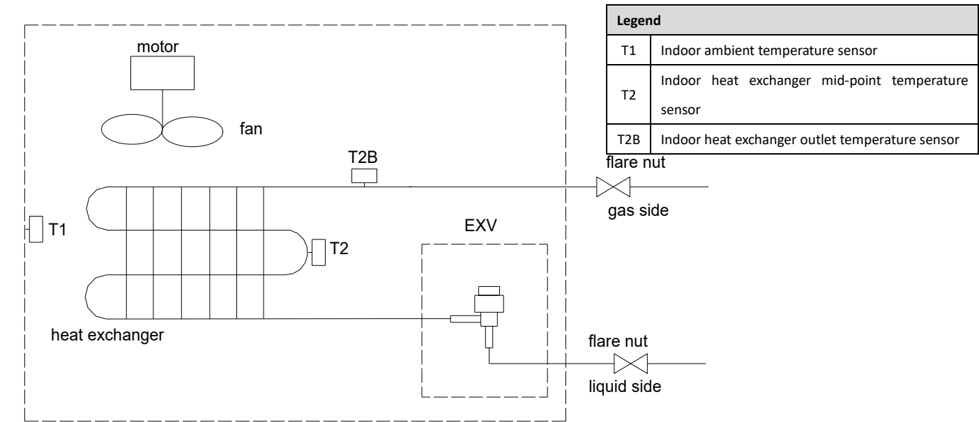
Figure 4.1: MDI2-71(80,90,112,140,160,200,250,280,400,450,560)T1DHN1 piping diagram
