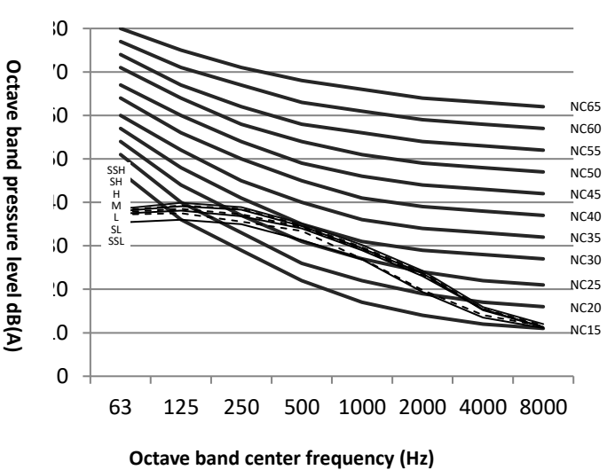
Figure 9.9: MDI2-560T1DHN1 octave band levels
