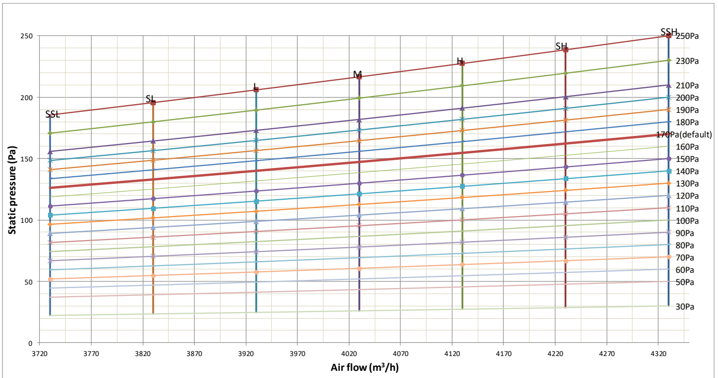
Figure 6.6: MDI2-200(250,280)T1DHN1 fan performance
