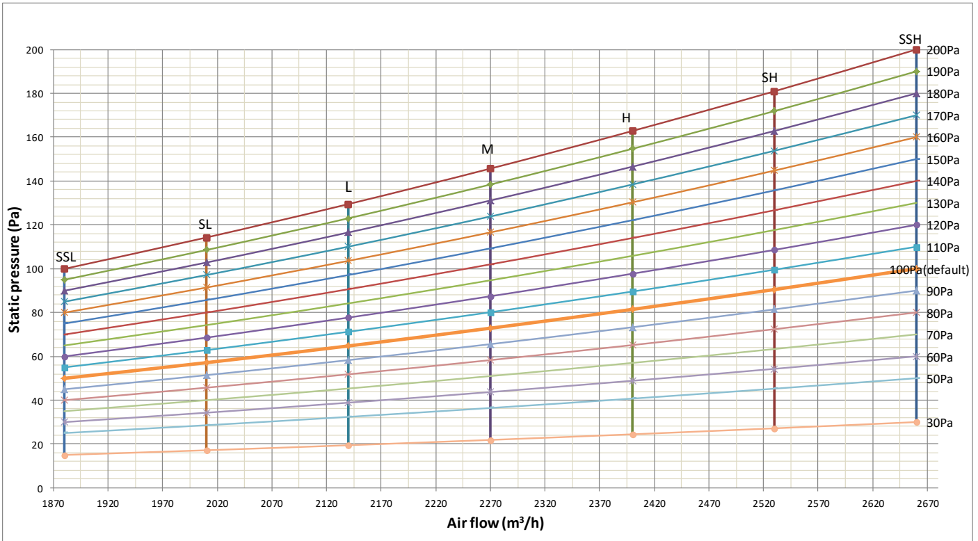
Figure 6.5: MDI2-160T1DHN1 fan performance
