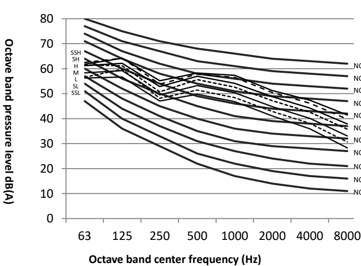
Figure 9.8: MDI2-400(450)T1DHN1 octave band levels
