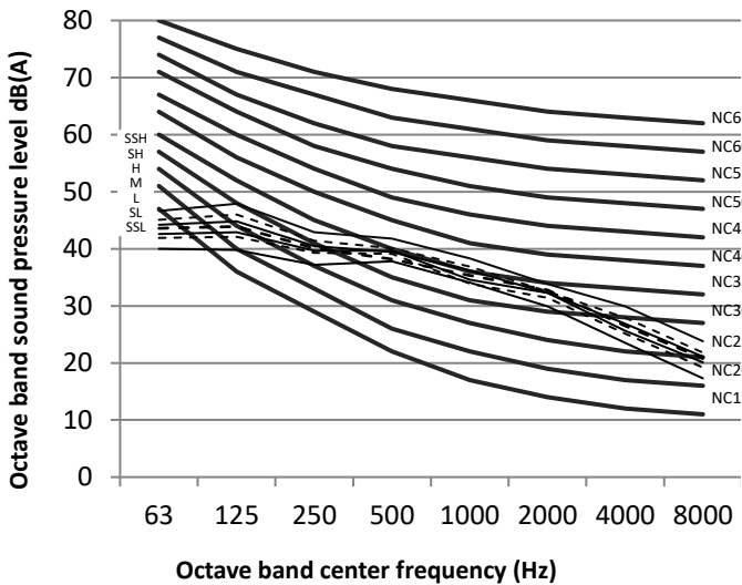
Figure 9.6: MDI2-160T1DHN1 octave band levels
