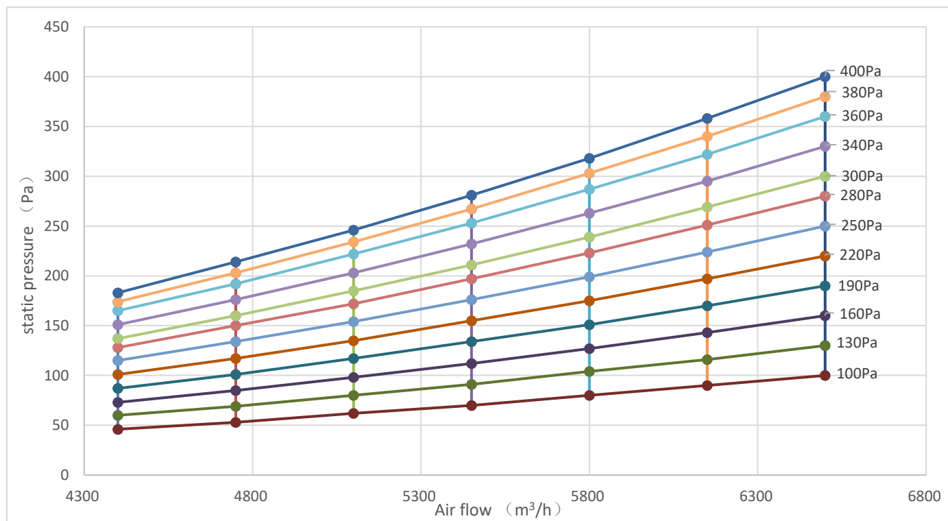
Figure 6.7: MDI2-400(450)T1DHN1 fan performance
