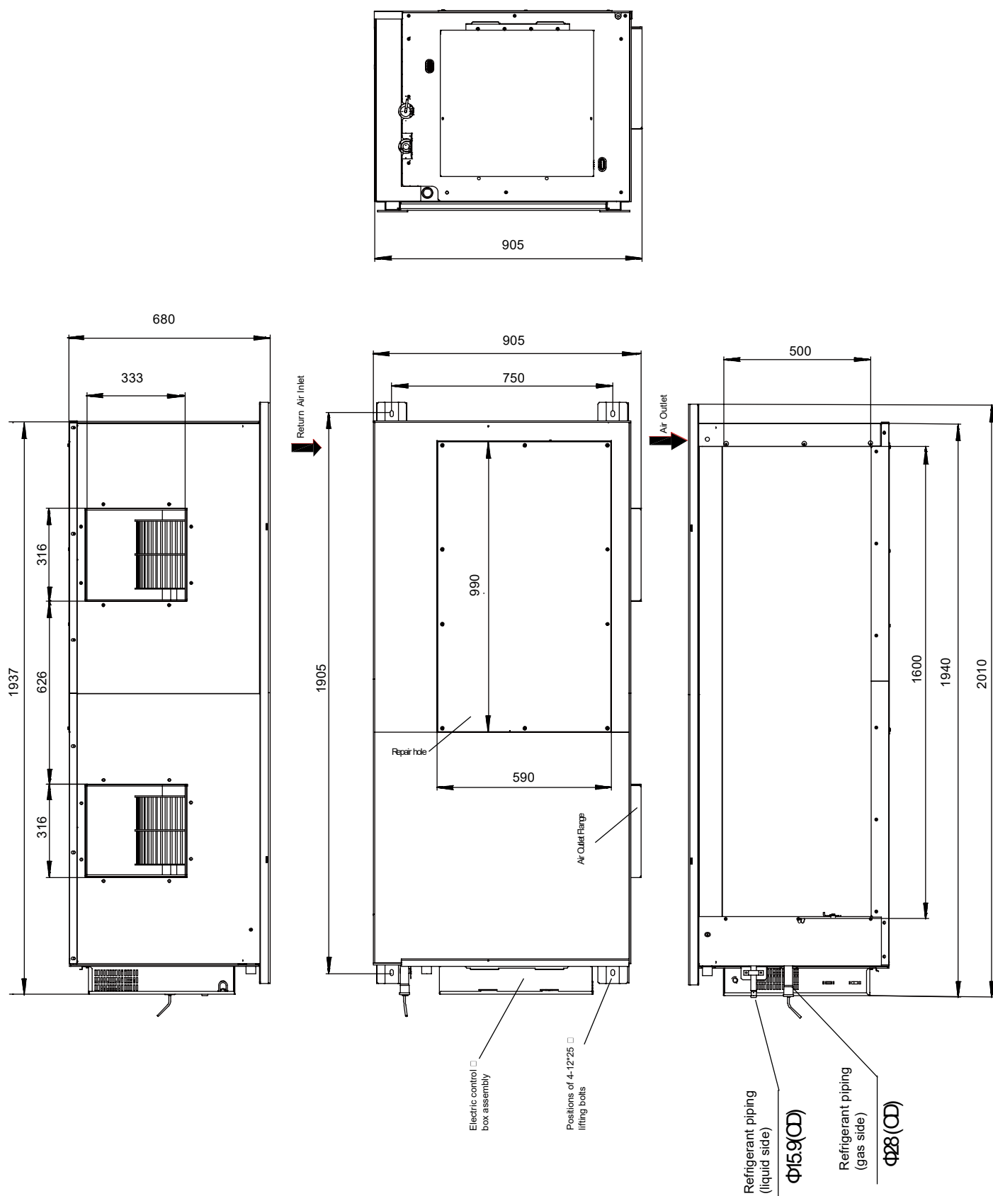
Figure 2.4: MDI2-400(450,560)T1DHN1 dimensions (unit: mm)
