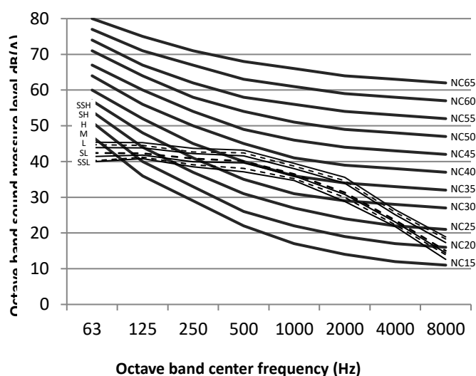
Figure 9.3: MDI2-90T1DHN1 octave band levels
